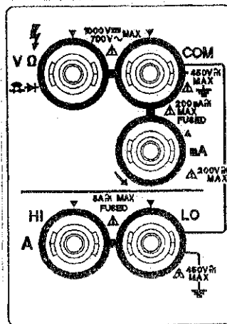
(b) R6441C
