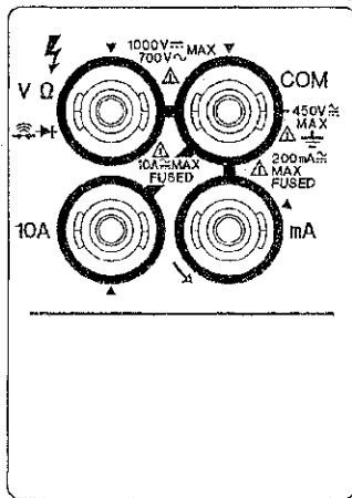
(a) R6441A/B
